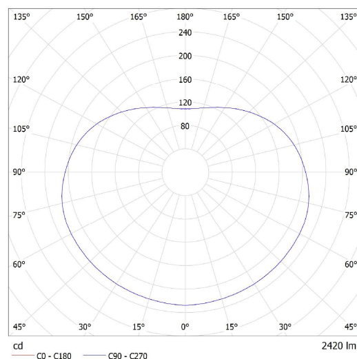
Lucis ZKS.L2.300.X POLARIS ZKS LED / LDC (Polar)
